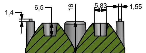
SECTION F-F
