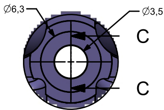
DETAIL B SCALE 5:1
