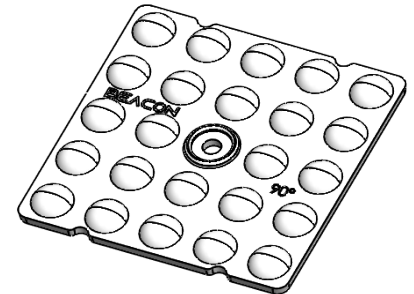
Isometric View
